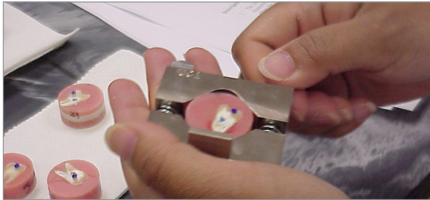
Sample held in test clamp
